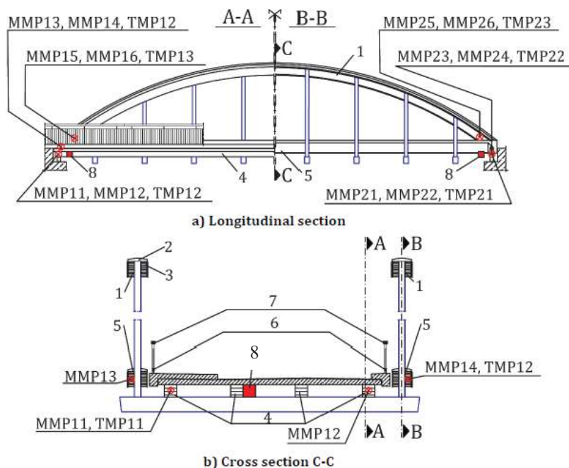
Figure 9. Moisture monitoring – example arch truss (according to Figure D.13 of [3])
