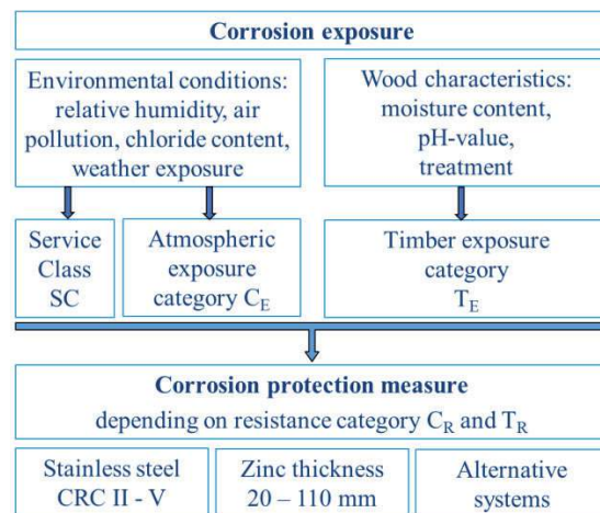
Figure 6. Procedure for selecting corrosion protection measures according to [3]
