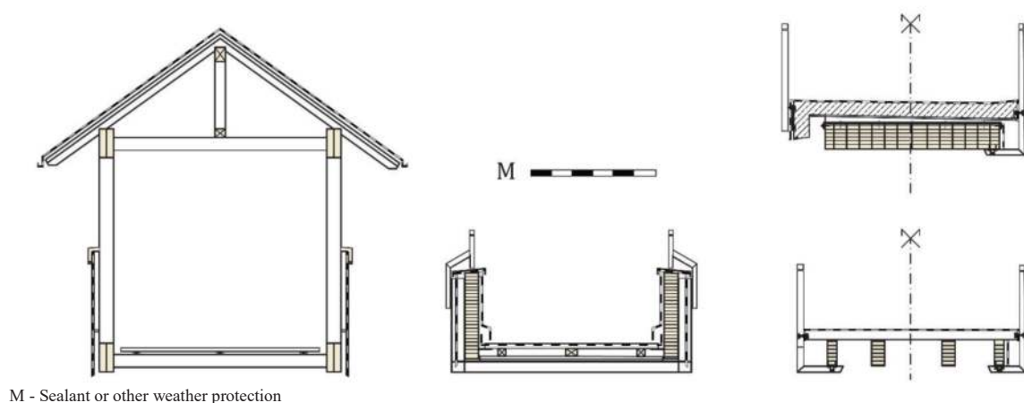
Figure 3. Types of bridge protection by roof overhang and water resistant layer: covered bridge (left), trough bridge (middle), 3 deck bridges (right) (according to Figure 3.1 of [3])
