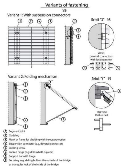
Figure 8. Examples of the construction of removable cladding [13]
