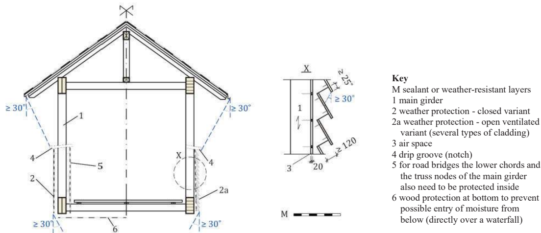
Figure 5. Construction measures: Weather protection by roof and planking [according to Figure D.3 of [3]]
